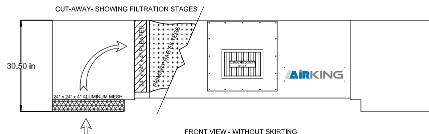
FRONT VIEW - WITHOUT SKIRTING
