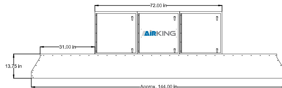
SIDE VIEW - WITH SKIRTING
