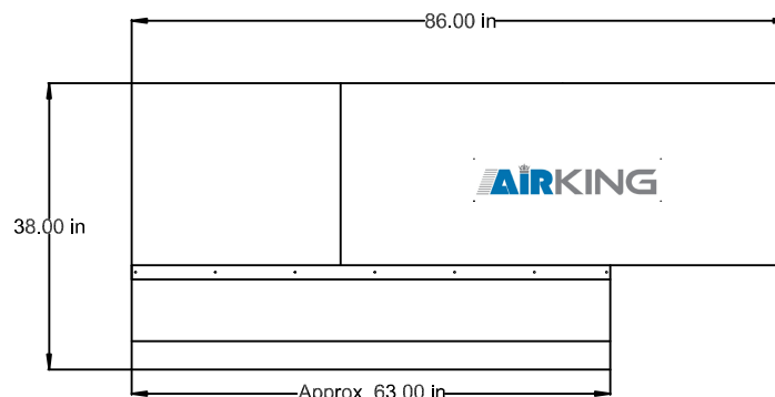
SIDE VIEW - WITH SKIRTING
