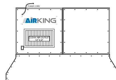
FRONT VIEW - WITH SKIRTING
