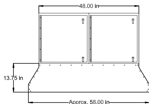
BACK VIEW - WITH SKIRTING
