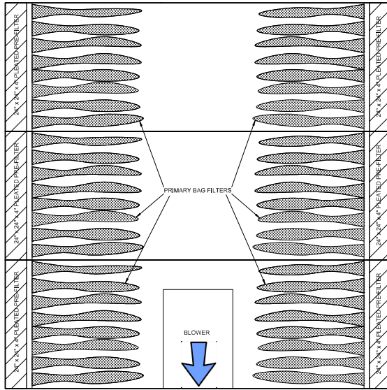
TOP VIEW : CUT-AWAY
