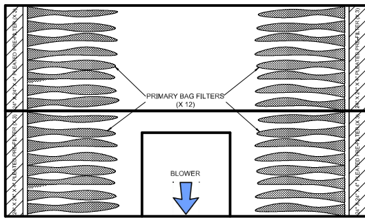
TOP VIEW : CUT-AWAY
