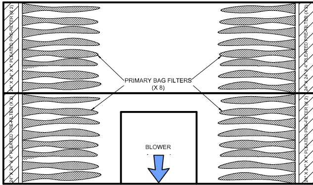
TOP VIEW : CUT-AWAY
