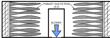
TOP VIEW : CUT-AWAY
