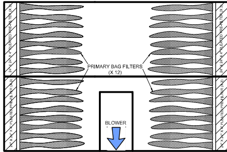
TOP VIEW : CUT-AWAY
