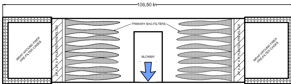
TOP VIEW : CUT-AWAY
