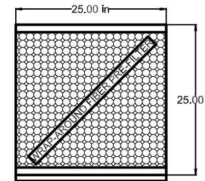
SIDE VIEW/ CAGE CLOSED
