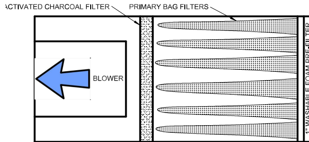
TOP VIEW : CUT-AWAY
