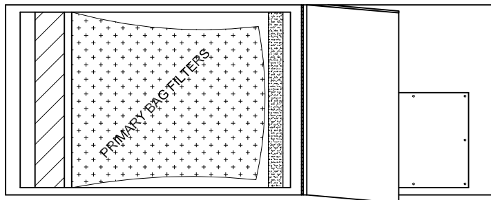
SIDE VIEW (FILTER ACCESS DOOR OPEN)
