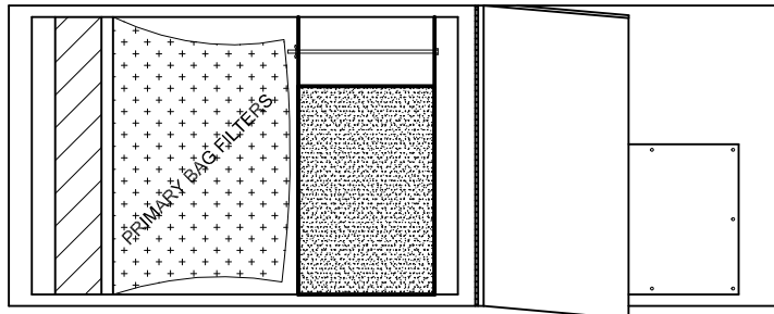
SIDE VIEW (FILTER ACCESS DOOR OPEN)
