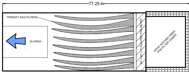
TOP VIEW : CUT-AWAY
