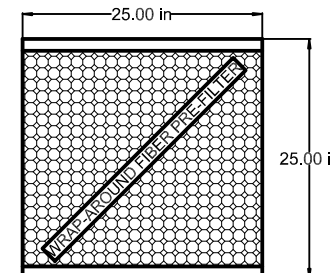
SIDE VIEW/ CAGE CLOSED
